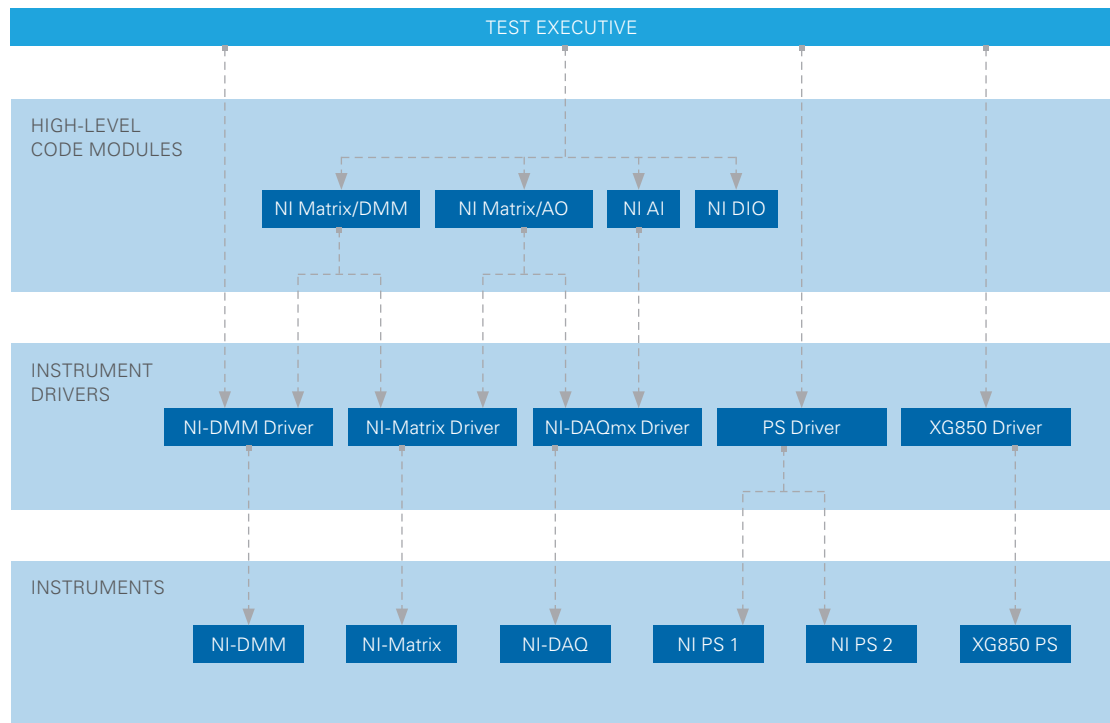
Figure 10. Overview of an Instrument-Specific Driver Method for Automated Test Software Without Abstraction
